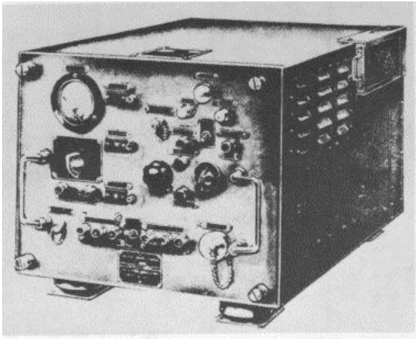
Receiver-Transmitter RT-38?()/uPI-12
